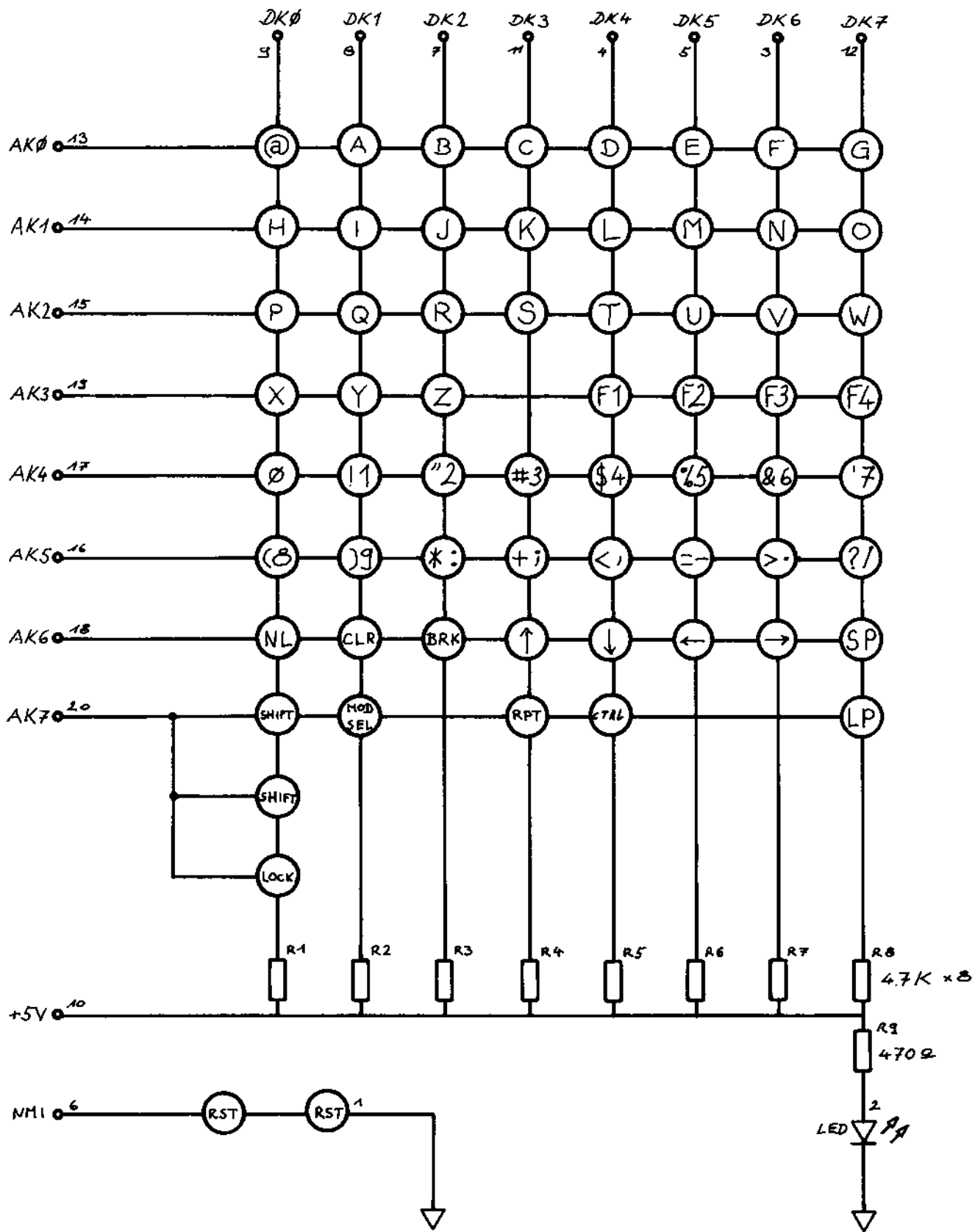
KEYBOARD CIRCUIT
