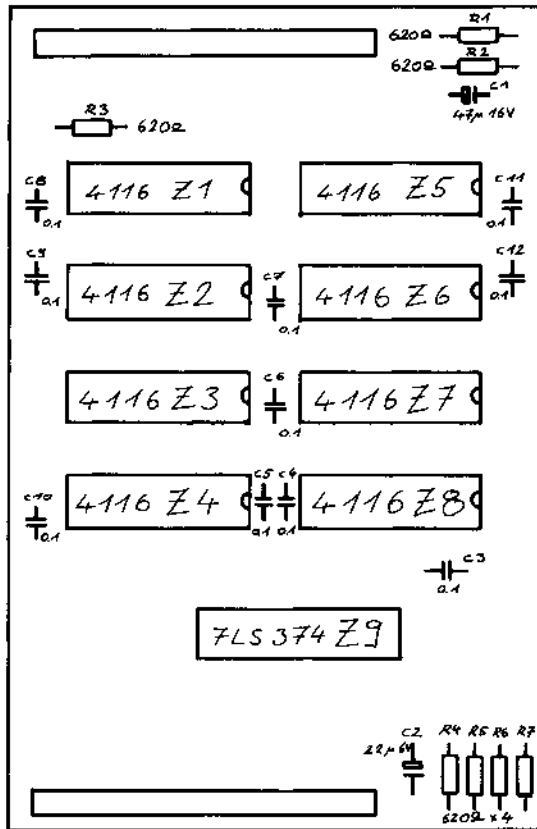
RAM ADAPTOR
